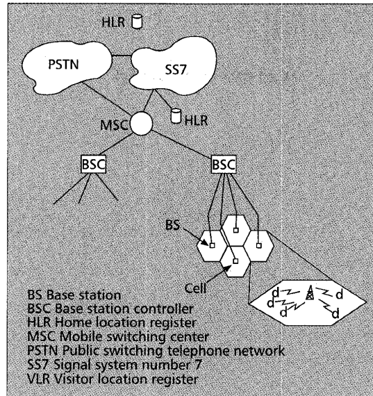
■ Figure 1. PCS network architecture.
